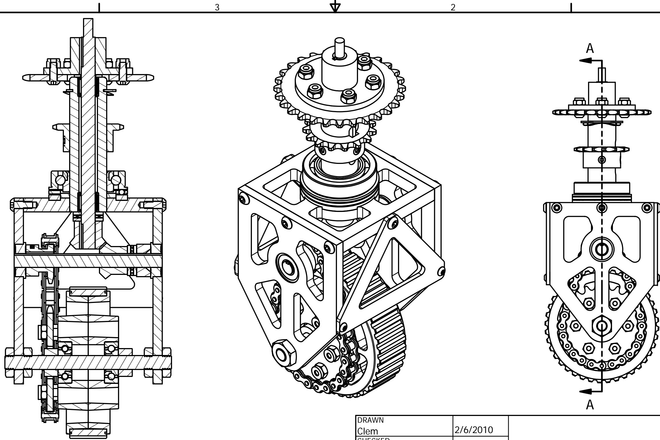
SECTION A-A SCALE 1 / 1.5
